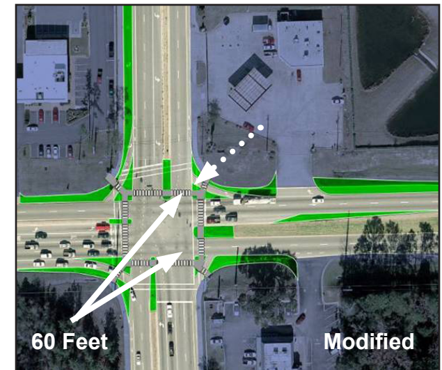
Crossing islands (pork chop islands) medians and more compact designs shorten pedestrian crossings to 30 seconds allowing motorists to be underway with less delay.
