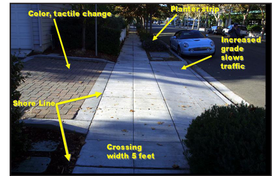
Typical Right-In, Right Out Crossing
