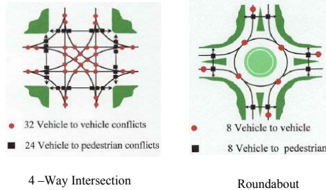
Possible Conflict Points: Roundabout vs. 4 Way Intersection
