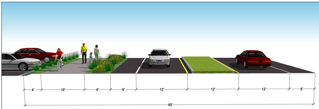
Highway 1 facing north is shown above, just north of 1st Street with the Coastal Trail and the northernmost parking lot for the restaurant on the left. The existing paved width is about 48 feet. This section is designed to fit within the existing width.
