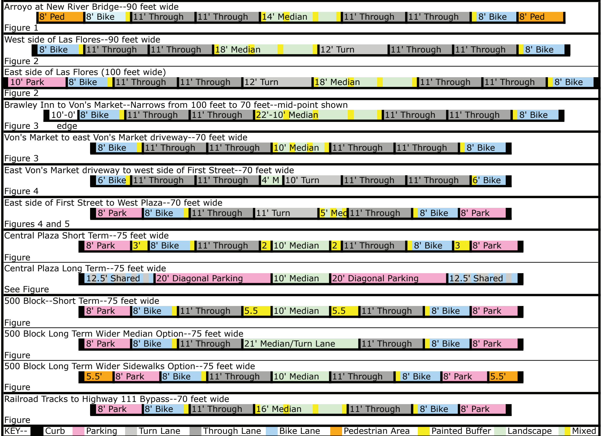
Figure 3-21 BRAWLEY MAIN STREET CROSS-SECTIONS
